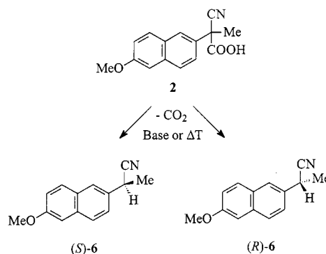
Scheme 3. Decarboxylation of 2 , leading to nitrile 6
