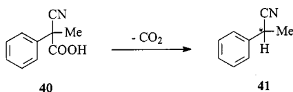
Scheme 7. Decarboxylation of 40 leading to nitrile 41
