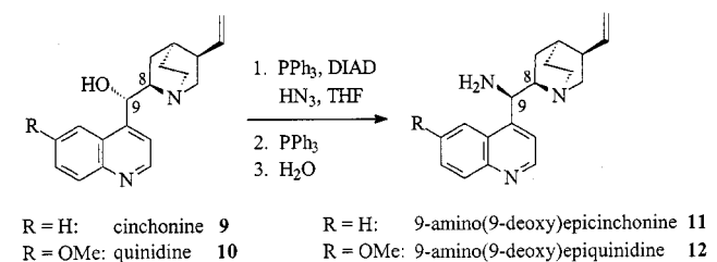
Scheme 5. Preparation of the 9-amino-9-deoxyepicinchona alkaloids 11 and 12
