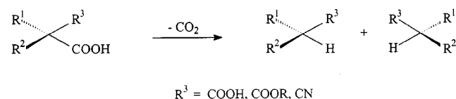
Scheme 1. Decarboxylation of malonic acids, their monoesters and cyanoacetic acids
