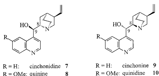
Figure 2. The cinchona alkaloids 7–10
