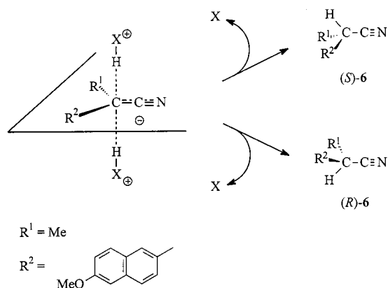
Scheme 4. Protonation of the planar ketenimine anion from the top face or the bottom face, leading to the different enantiomers of nitrile 6
