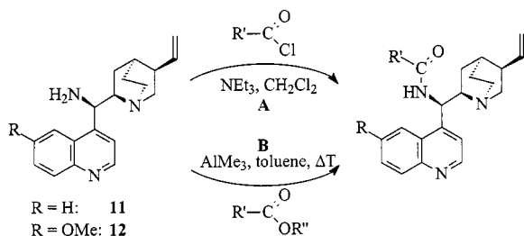
Scheme 6. Preparation of amides from amines 11 and 12 and either carboxylic acid chlorides (method A) or trimethylaluminum and carboxylic acid esters (method B)
