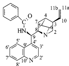
Figure 3. N -(9-Deoxyepicinchonine-9-yl)benzamide ( 13 )
