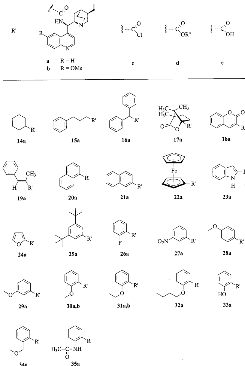
Figure 4. Amides a of 11 and b of 12 , synthesized according to method A or B, and the carboxylic acid chlorides c , carboxylic esters d , and carboxylic acids e
