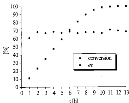
Figure 6. Kinetics of the decarboxylation of 2 with base 31a
