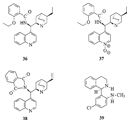
Figure 5. Additional bases tested in the decarboxylation of 2
