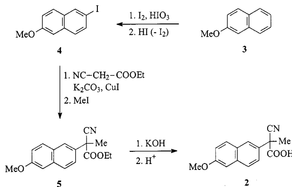
Scheme 2. Preparation of the substrate 2
